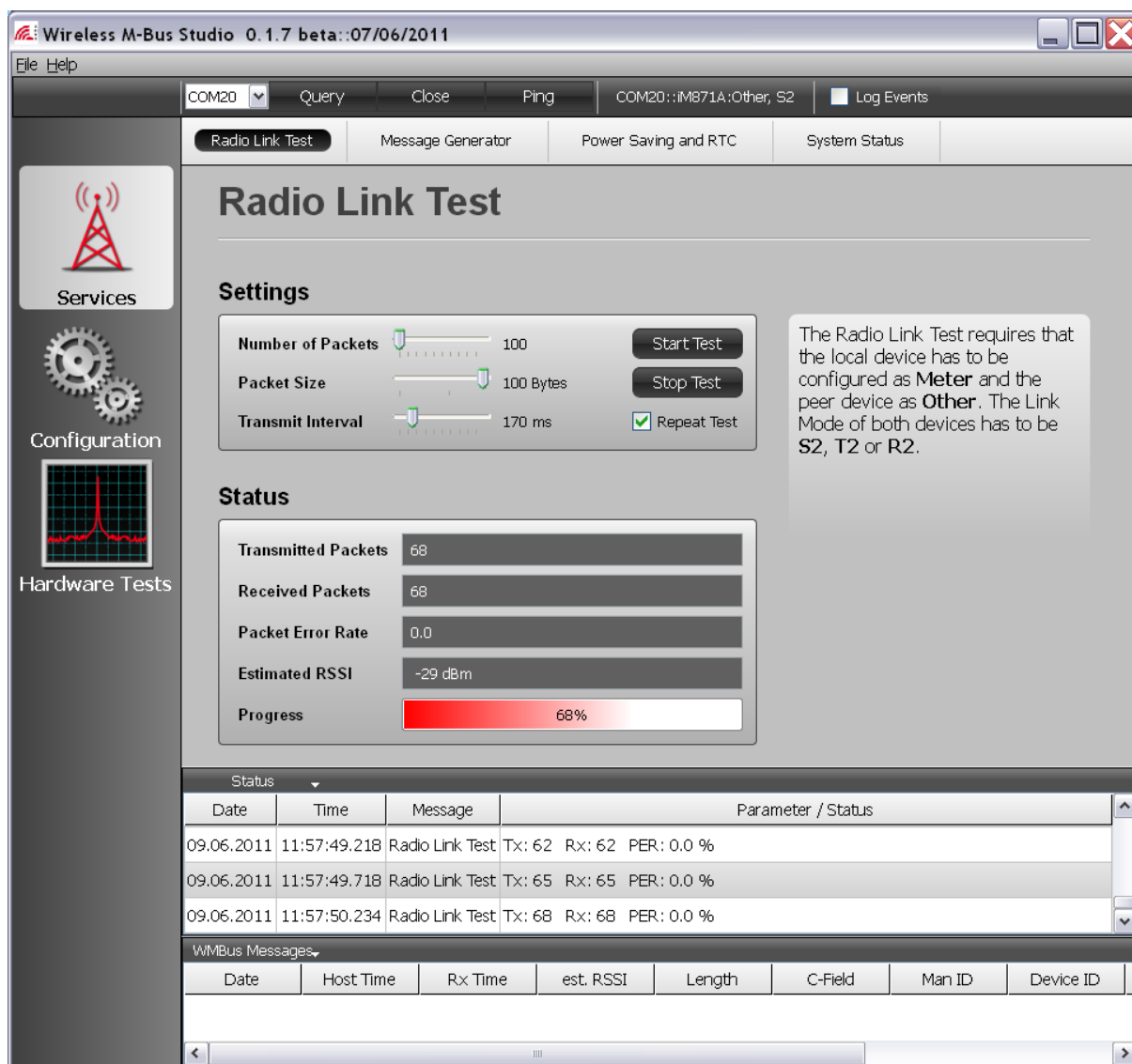
Figure 3-2: Radio Link Test
